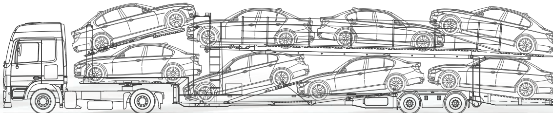
Loading example ruslan® with 4,00 m height. Observe national regulations!
