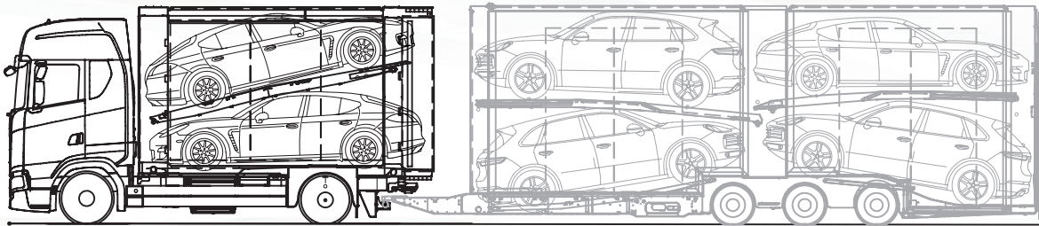
Loading example ecomode performance S2-180 combined with ecomode performance T4-235 with 4 m height. Observe national regulations!
