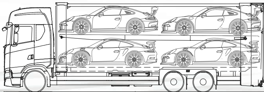
Loading example ecomode performance S4-260 L with 4,00 m height. Observe national regulations!
